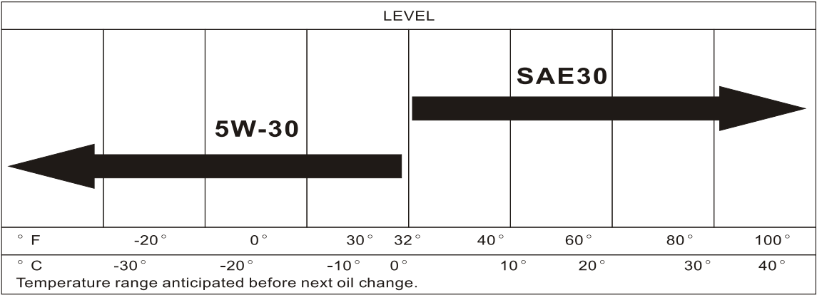
LUBRICATION CHART
