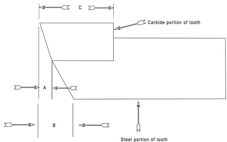
Fig. 15: Guide to sharpening grinding teeth
