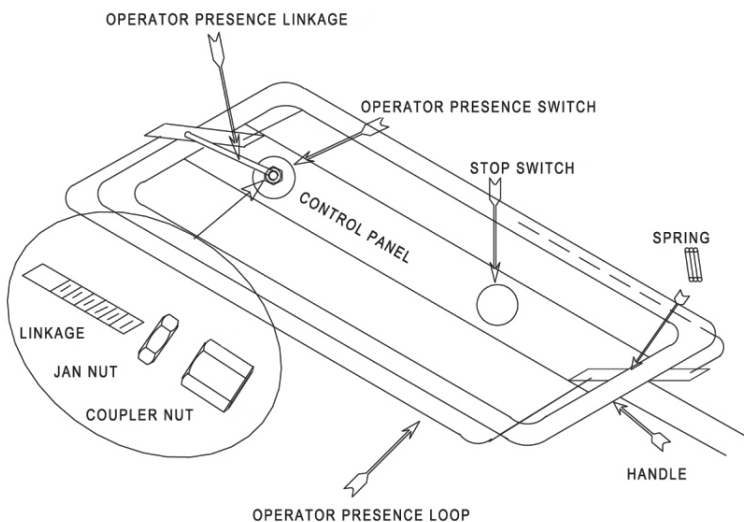
Fig. 8 Operatorpresence system
