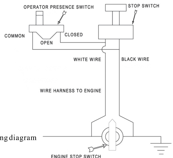
Fig. 8 Operatorpresence system
