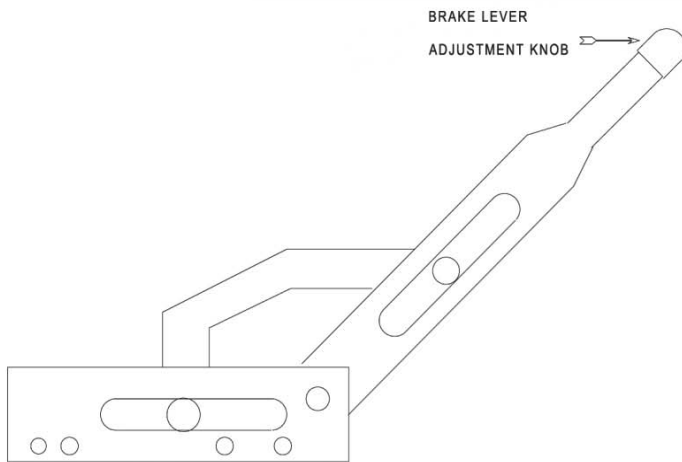
Fig. 10: Brake lever adjustment.
