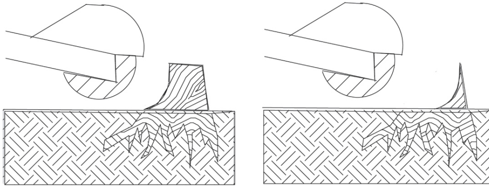
Fig.7: Stump grinding below ground level
